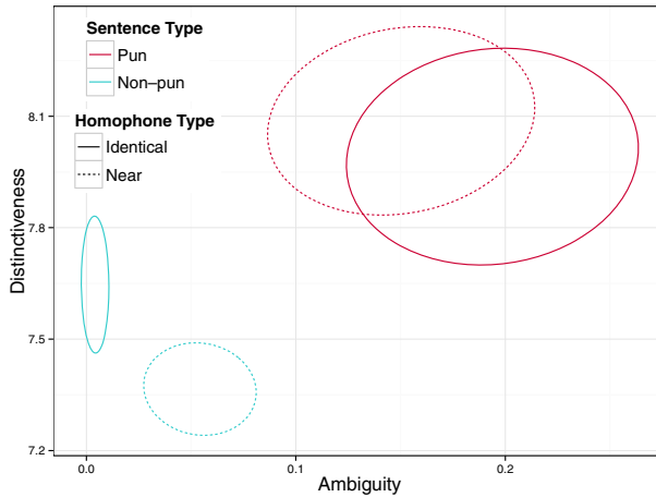
Fig. 2. Standard error ellipses of ambiguity and distinctiveness for each sentence type. Puns (both identical and near homophone) score higher on ambiguity and distinctiveness; non-pun sentences score lower.
