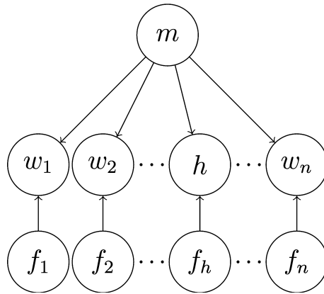
Fig. 1. Graphical representation of a generative model of a sentence. If the indicator variable f_i has value 1, w_i is generated based on semantic relatedness to the sentence meaning m ; otherwise, w_i is sampled from a trigram language model based on the immediately preceding two words.
